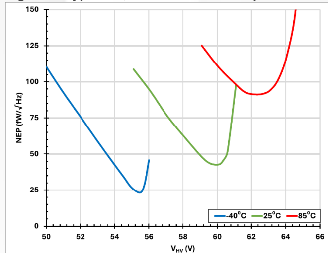
Figure 6. Typ. NEP, R_L = 50 \Omega Area = 80 \mu\text{m}
