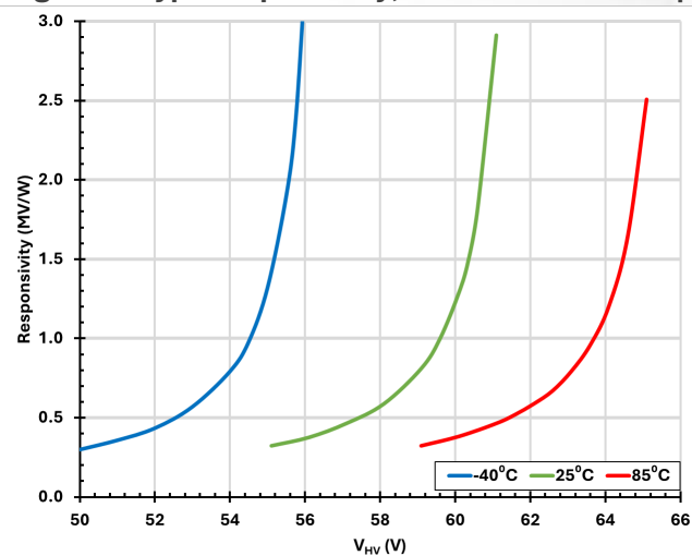
Figure 5. Typ. Responsivity, R_L = 50 \Omega Area = 80 \mu\text{m}
