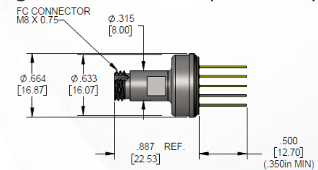
Figure 11. FC connector (617-339814)
