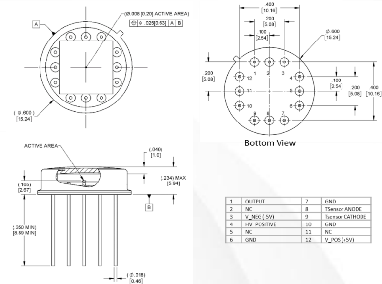
Figure 6. Package Dimension and Pinout
