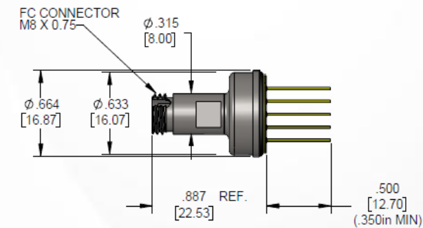
Figure 7. FC connector (617-339834)
