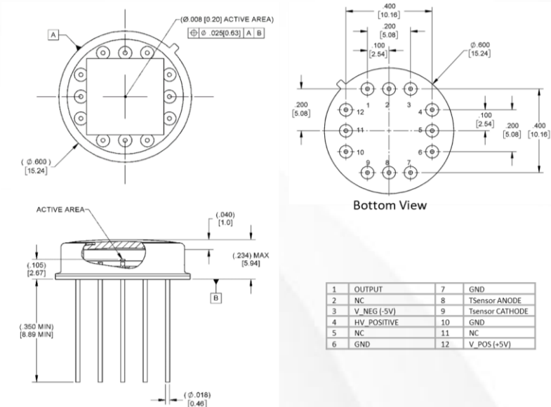
Figure 6. Package Dimension and Pinout
