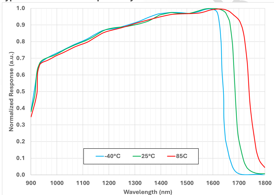
Figure 1. Typical Normalized Responsivity
